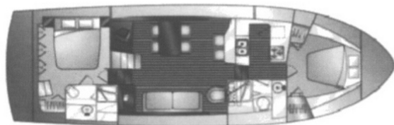
2-Stateroom Layout
